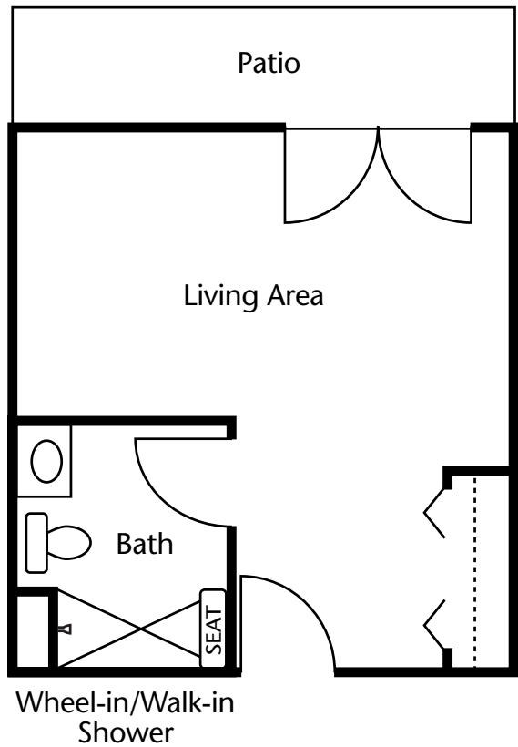
Studio with Patio - Handicap Accessible 398 sq. ft.
