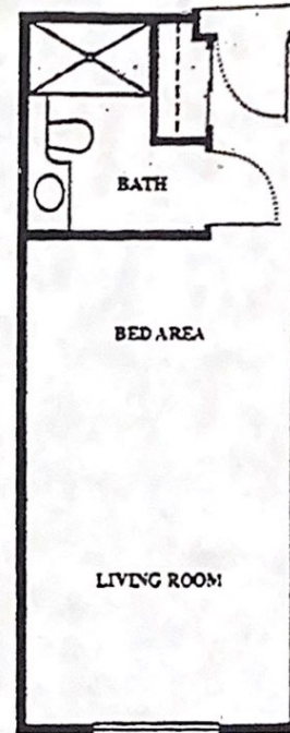
Plan B Typical Efficiency Unit (Approx. 330 Sq. Ft.)
